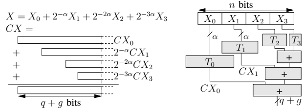
Fig. 2. The KCM LUT-based method
